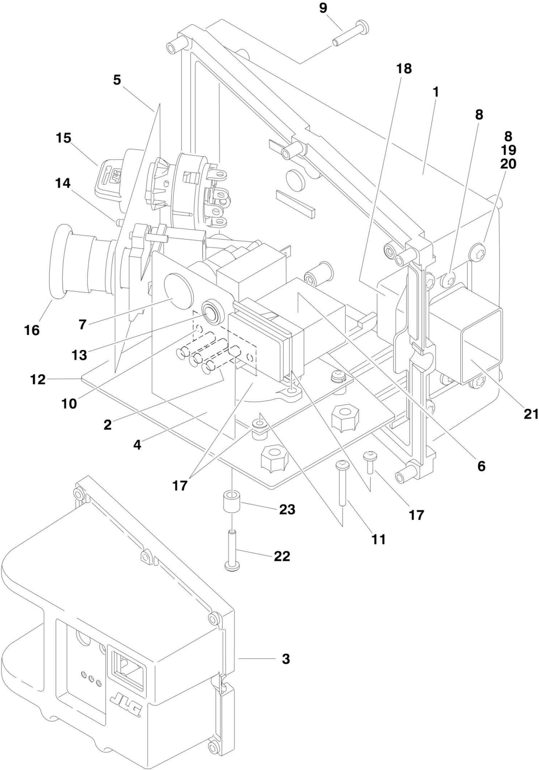
FIGURE 2-4. GROUND CONTROL ASSEMBLY (MACHINES WITH 100112456 DRIVE MODULE)
